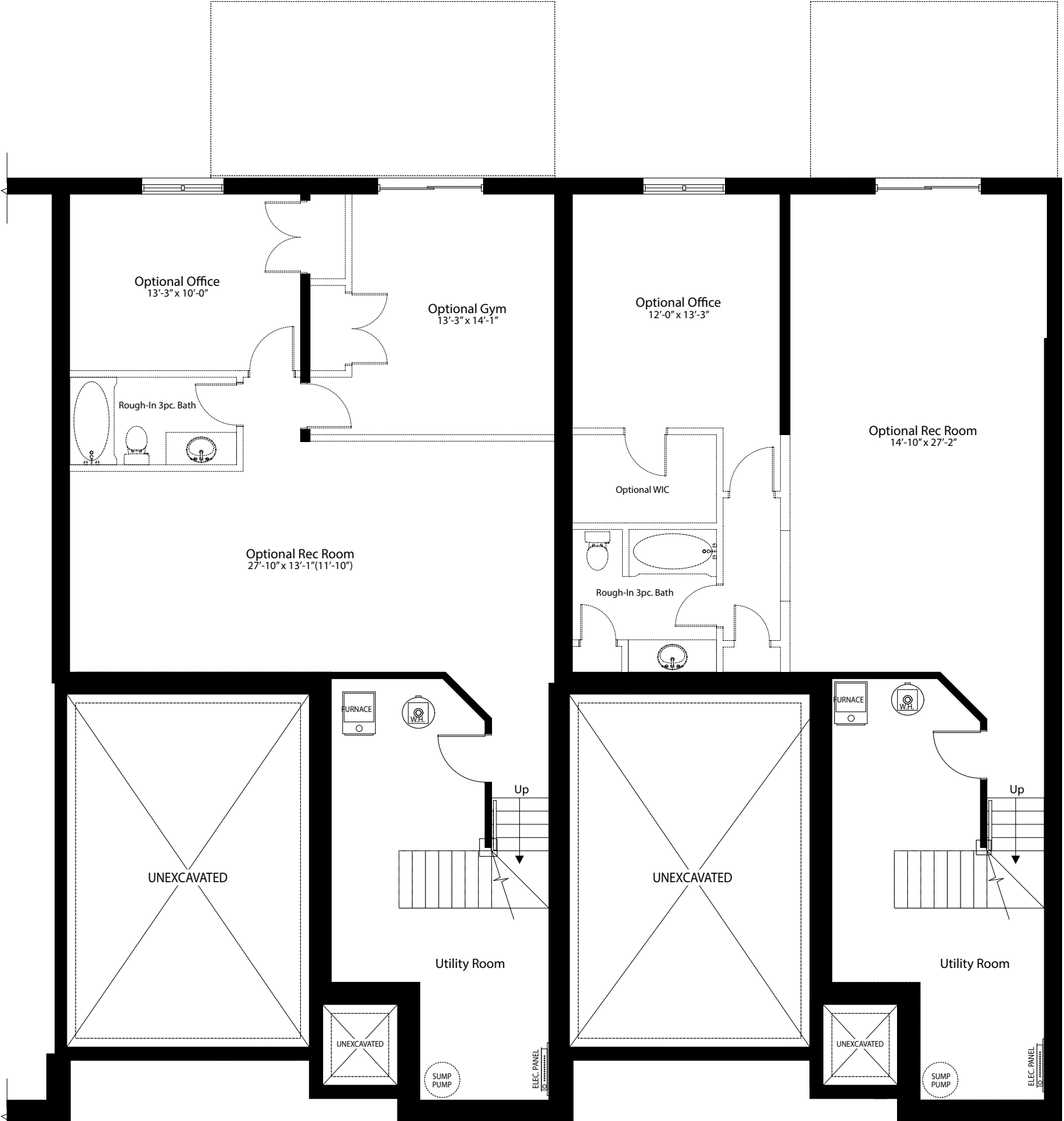
FOUNDATION PLAN
